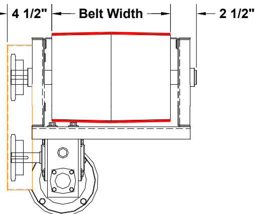
Standard Drive Cross Section
