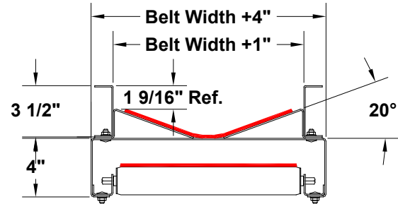
Standard Frame Cross Section
