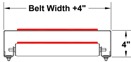
Standard Frame Cross Section
