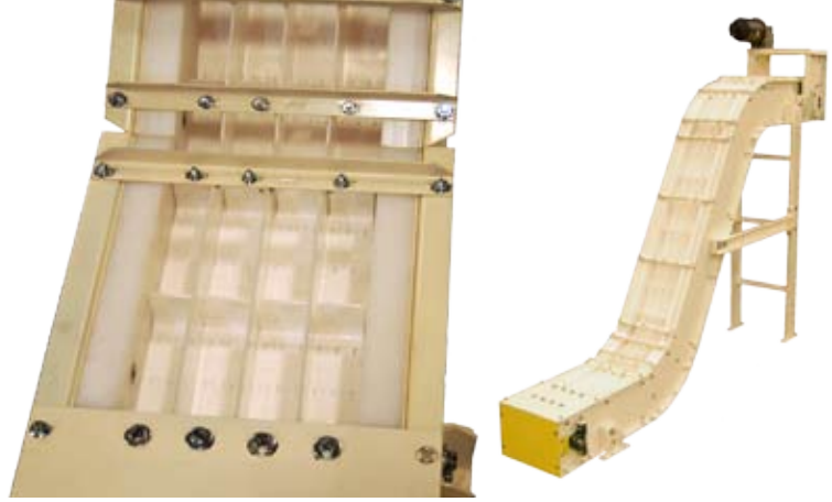
Titan designed and built plastic belt conveyor with 4 lanes for transporting colored plastic pellets to packaging
