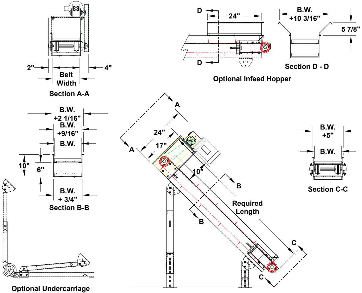
Dimensions for Optional Undercarriage
