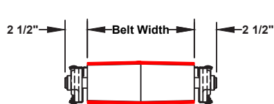
Standard Infeed Cross Section
