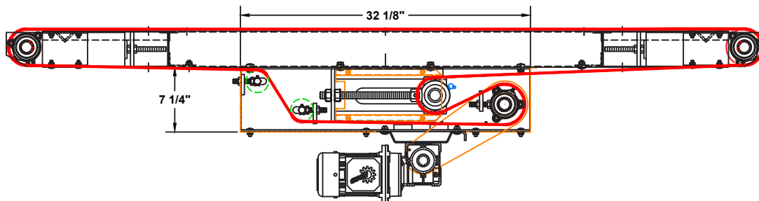
STANDARD CENTER DRIVE & TAKE-UP
