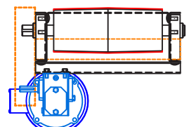
STANDARD BOTTOM MOUNT DRIVE CROSS SECTION
