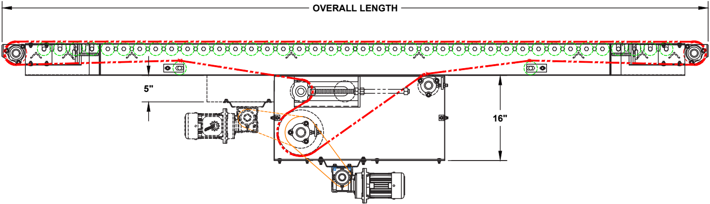
Center Drive and Take-up
