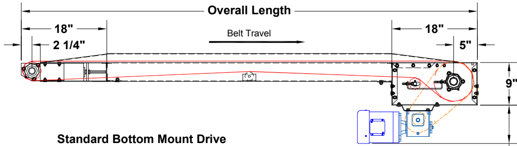
Standard Bottom Mount Drive
