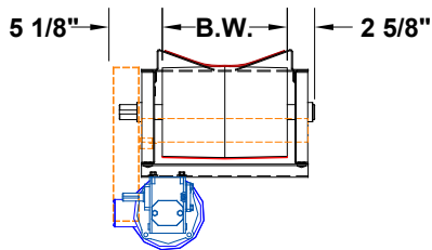
Standard Drive Cross Section
