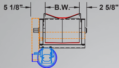
Standard Drive Cross Section
