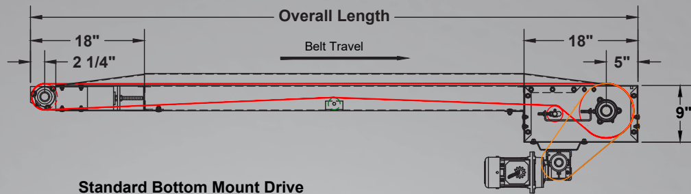
Standard Bottom Mount Drive
