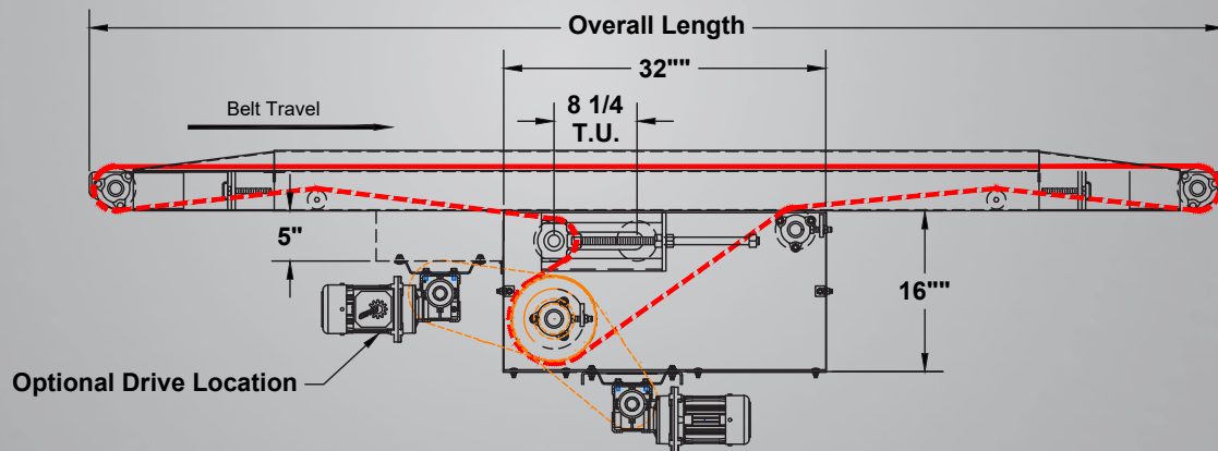
Standard Center Drive & Take-Up
