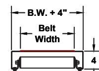
Standard Frame Cross Section
