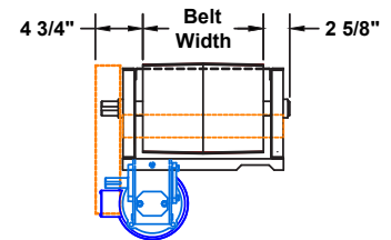
Standard Drive Cross Section
