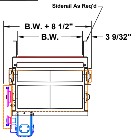
Standard Center Drive & Take-up Cross Section
