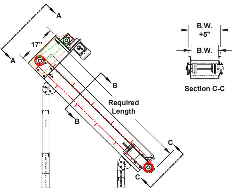
Dimensions for Optional Undercarriage
