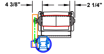
Section C - C Std. Bottom Mount Drive
