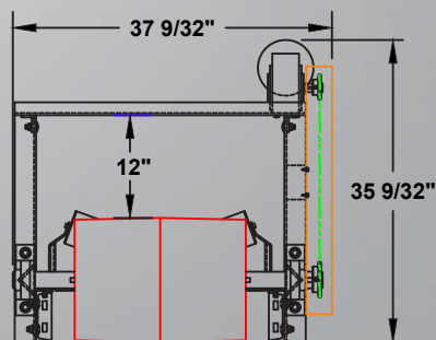
Top Mount Drive
