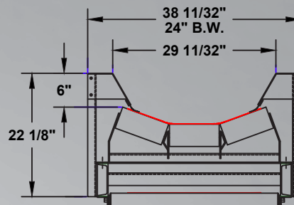
Typical Cross Section With Optional Siderail
