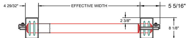
DOUBLE DRIVE GUARD (STANDARD CENTERS - 2 13/16")
