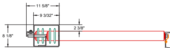
DOUBLE WIDE CHAIN GUARD (STANDARD CENTERS - 3 7/16")
