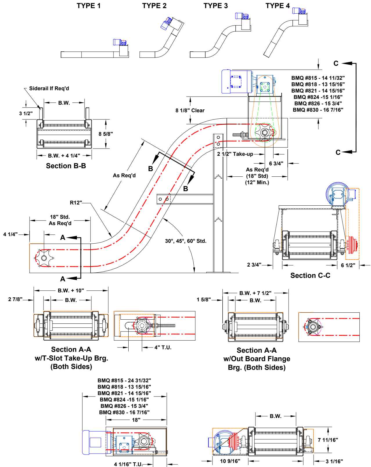
Optional Side Mount Drive
