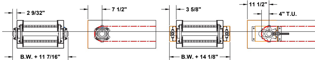
Section A - A w/Std. 4 Bolt Flange Brg.
