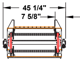
INFEED SECTION
