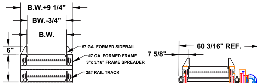
INCLINE SECTION
