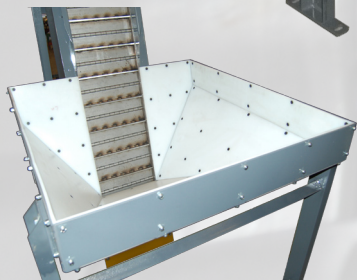
Custom hopper for delicate parts
