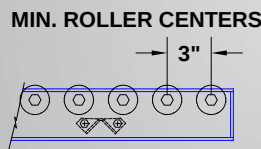
MODEL 425
