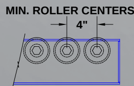
MODEL 435
